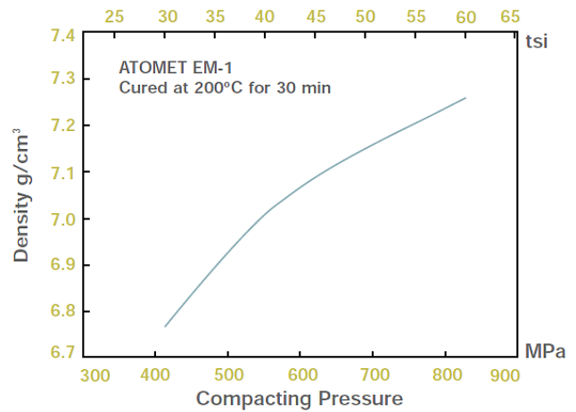
Compressibility
