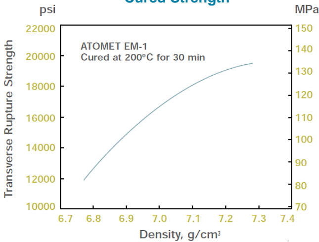
Cured Strength
