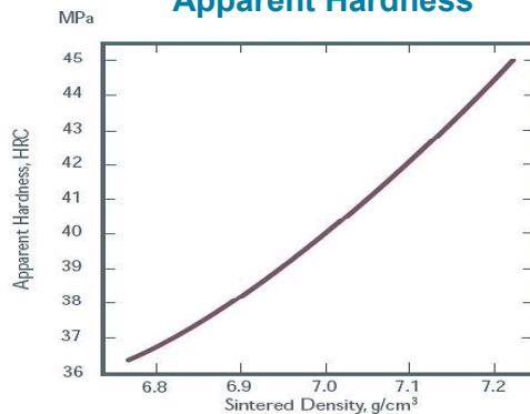
Apparent Hardness
