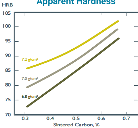
Apparent Hardness
