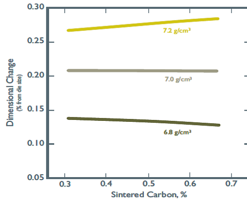
Dimensional Change
