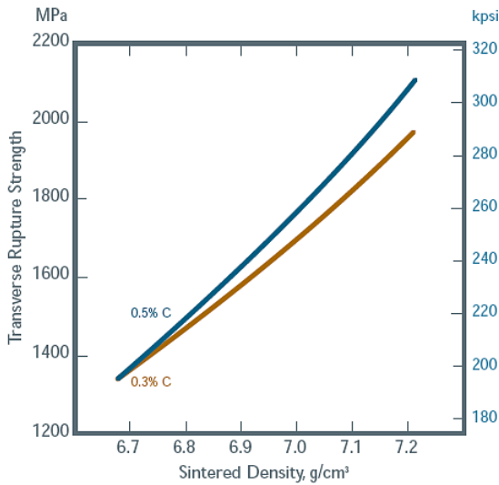
Transverse Rupture Strength
