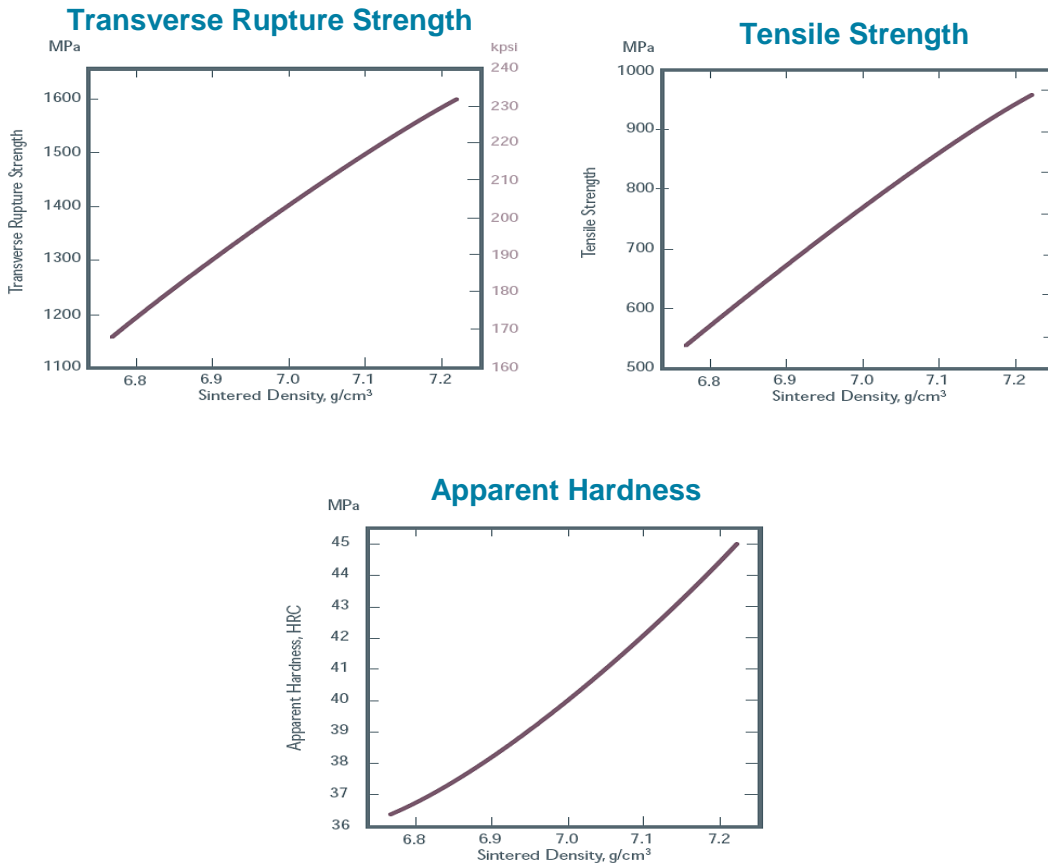
ATOMET 4001 + 0.55% graphite
