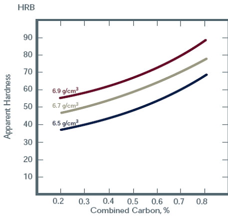
Apparent Hardness
