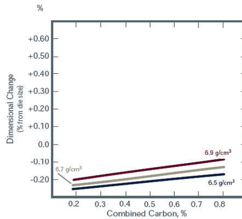
Dimensional Change
