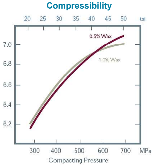
ATOMET 29 + Wax
