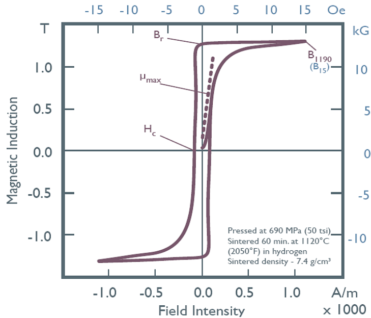
Hysteresis Curve
